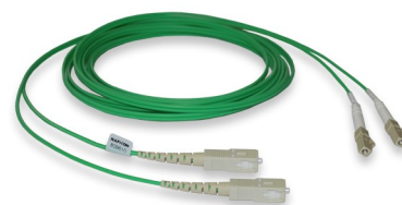
SC-UPC/LC-UPC OM1 DUPLEX
